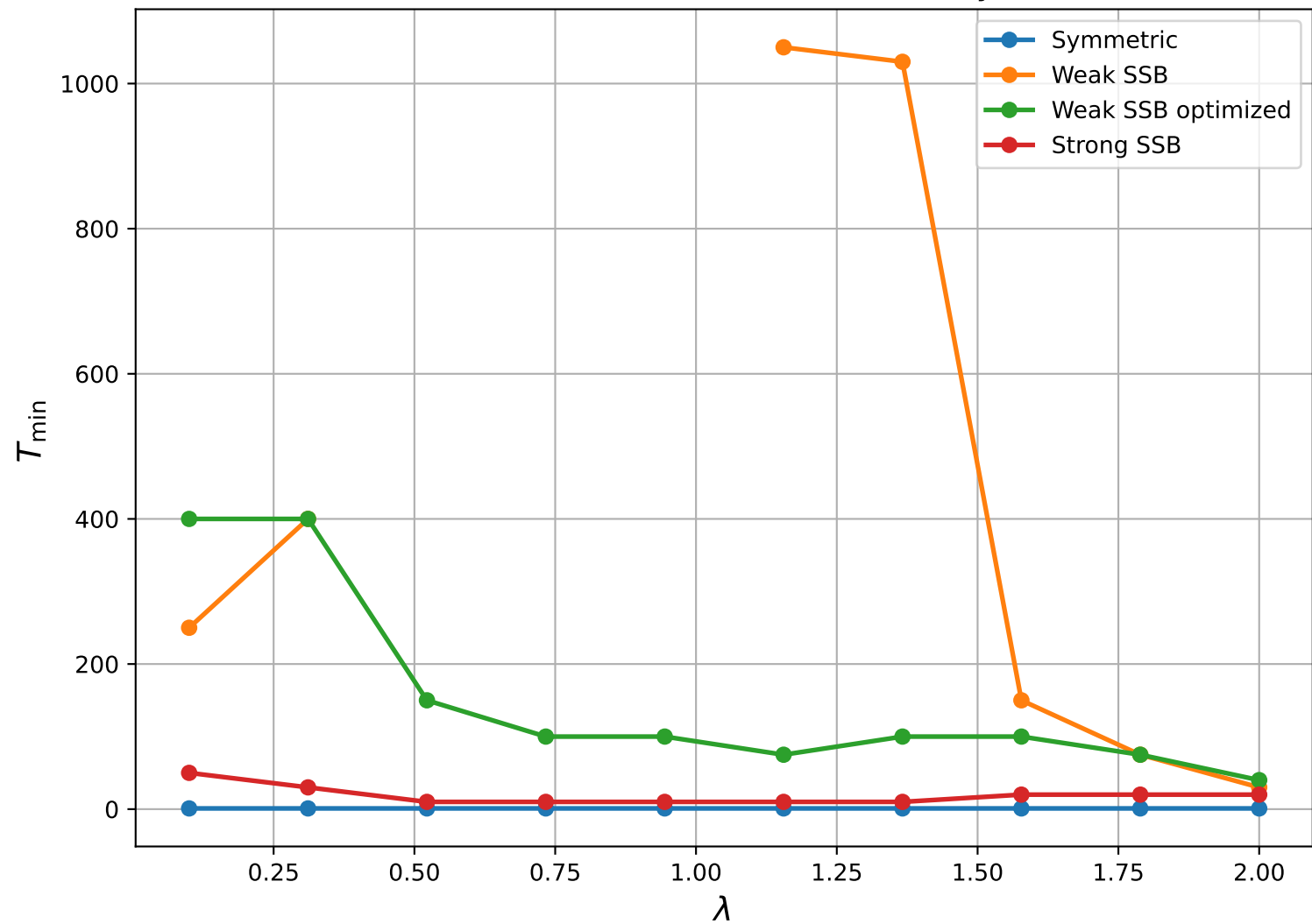
Minimum Adiabatic Time T_{\min} for Fidelity \geq 0.97
